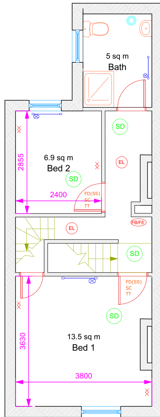
FIRST FLOOR
